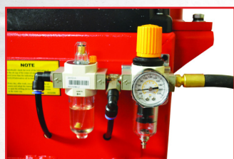
FILTER - REGULATOR - LUBRICATOR
